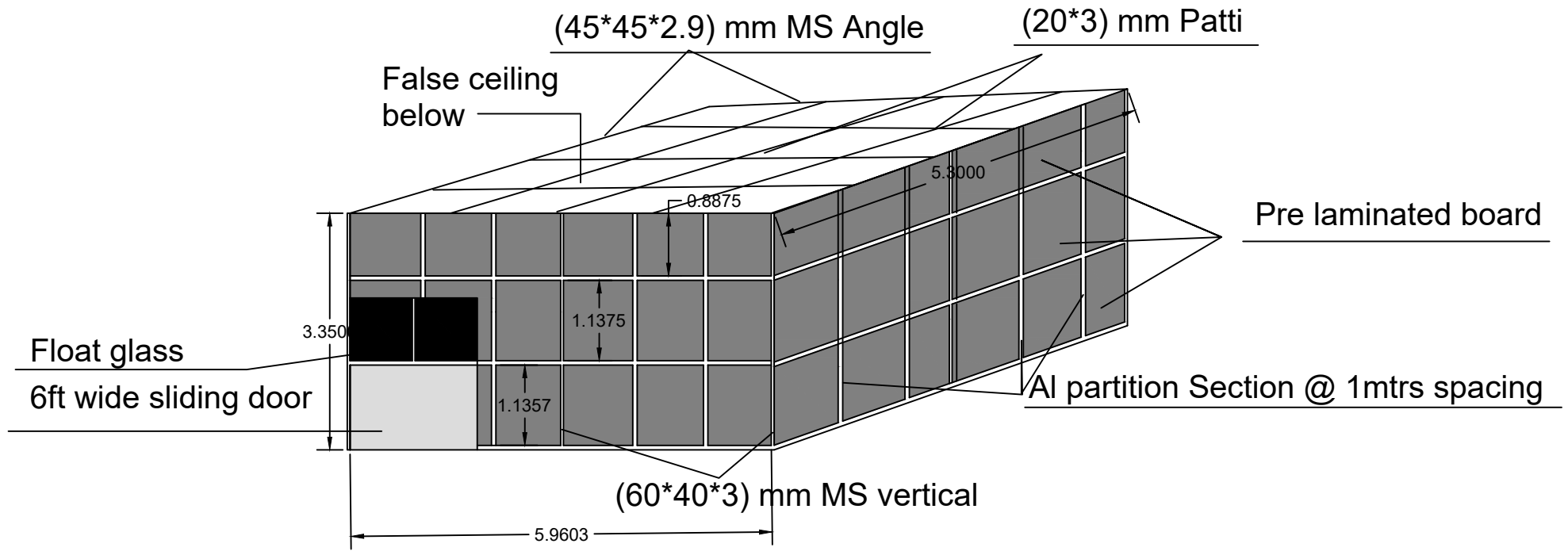
3D view for AI Partitioning and false ceiling work at new Mechanical Workshop
